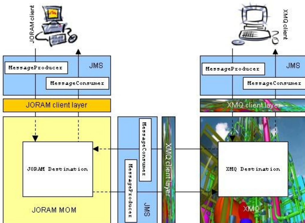
Figure 38 - Bridge communication diagram
