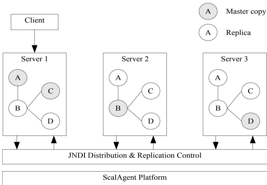
Figure 30 - JNDI replication
