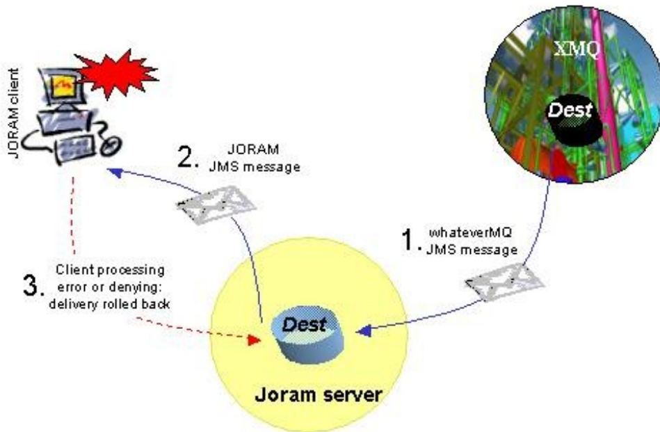
Figure 40 - Delivery rolled back by the JORAM client application
