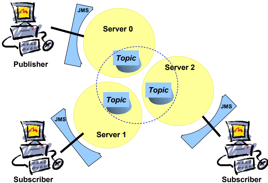
Figure 24 - Cluster sample configuration
