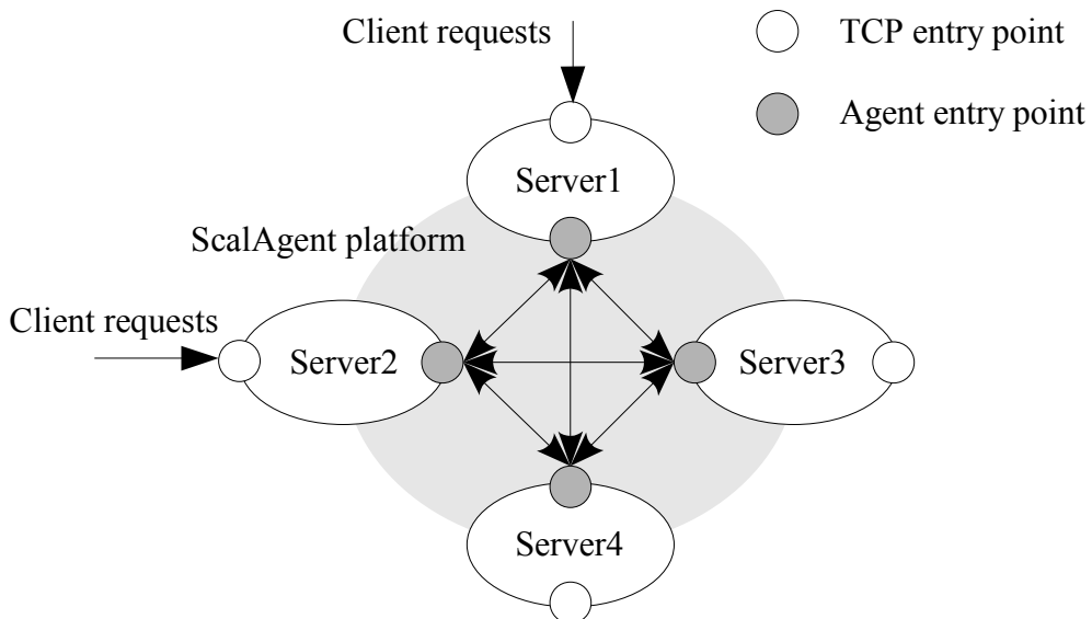
Figure 33 - Distributed configuration
