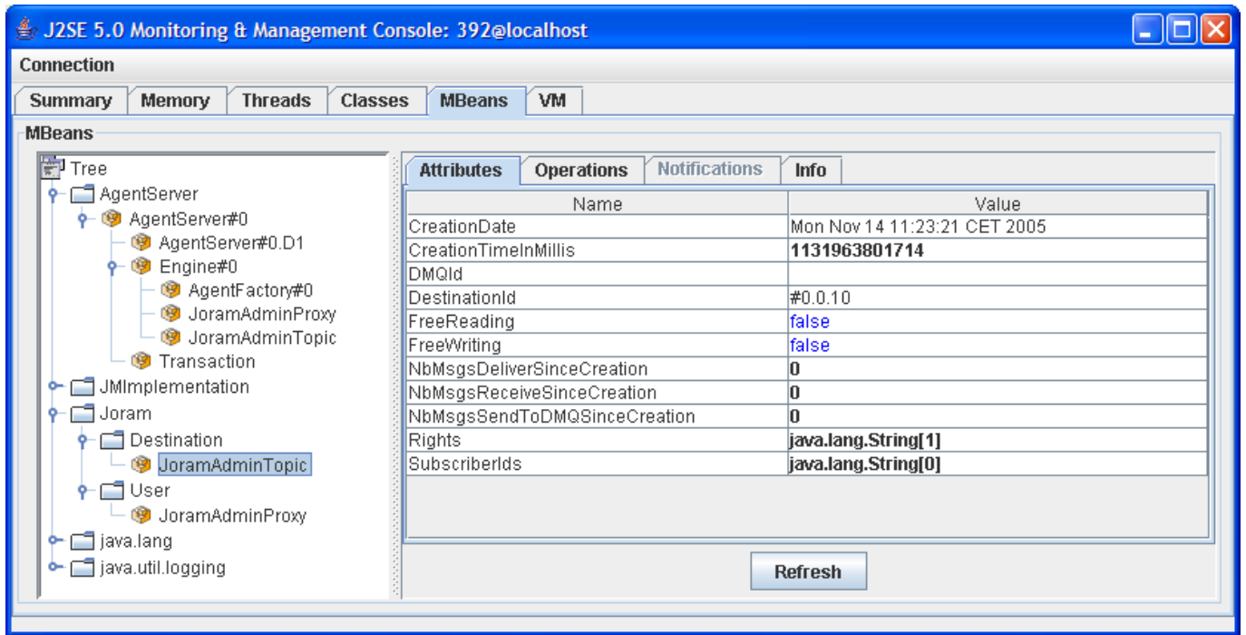
Jconsole View
