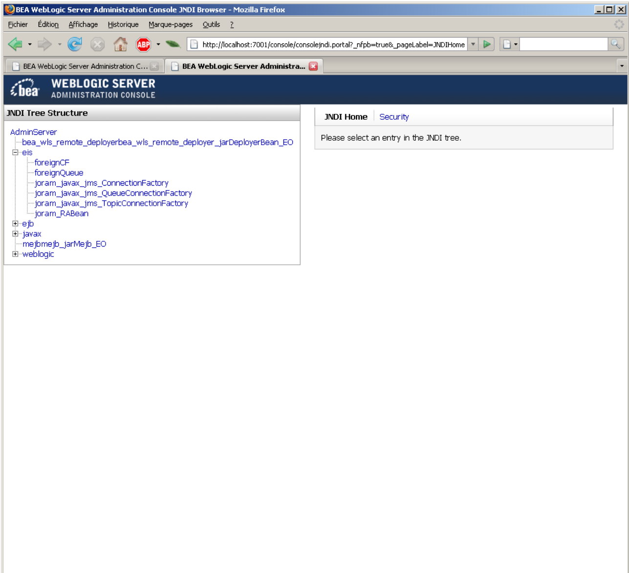
JNDI view
