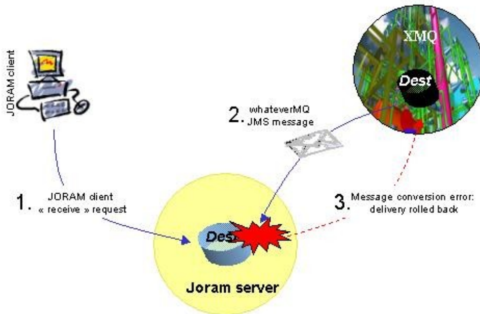
Figure 39 - Delivery rolled back by the JORAM bridge destination
