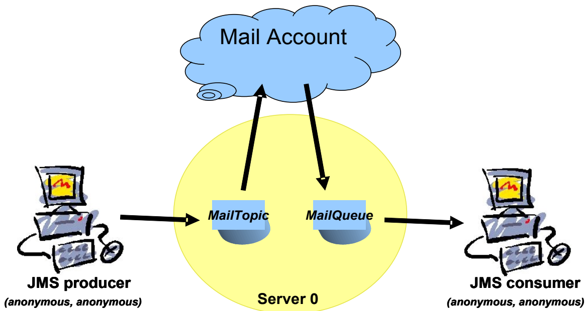
Figure 26 - The mail sample
