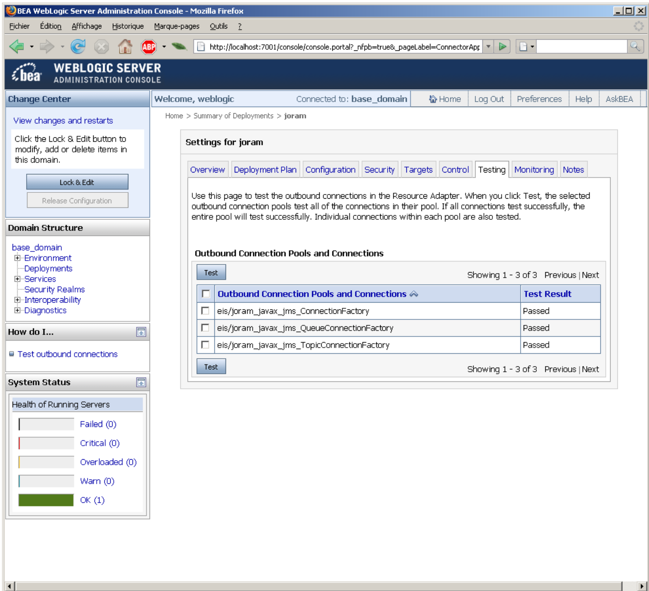
Joram RA tests view
