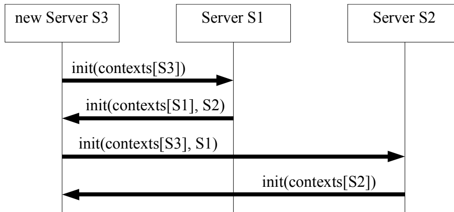
Figure 34 - Adding a new server
